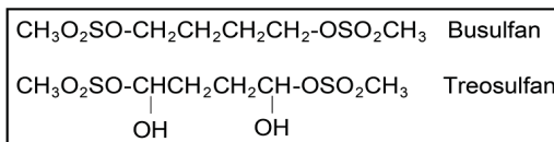
Figure 2: Molecular structures of busulfan and Treosulfan
